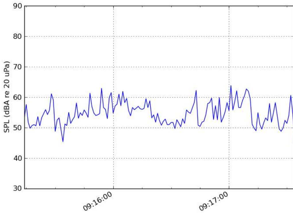
Figure 2.12. Sound Pressure Level at 23907 Sunvista During Play (Players on West Tennis Court)
